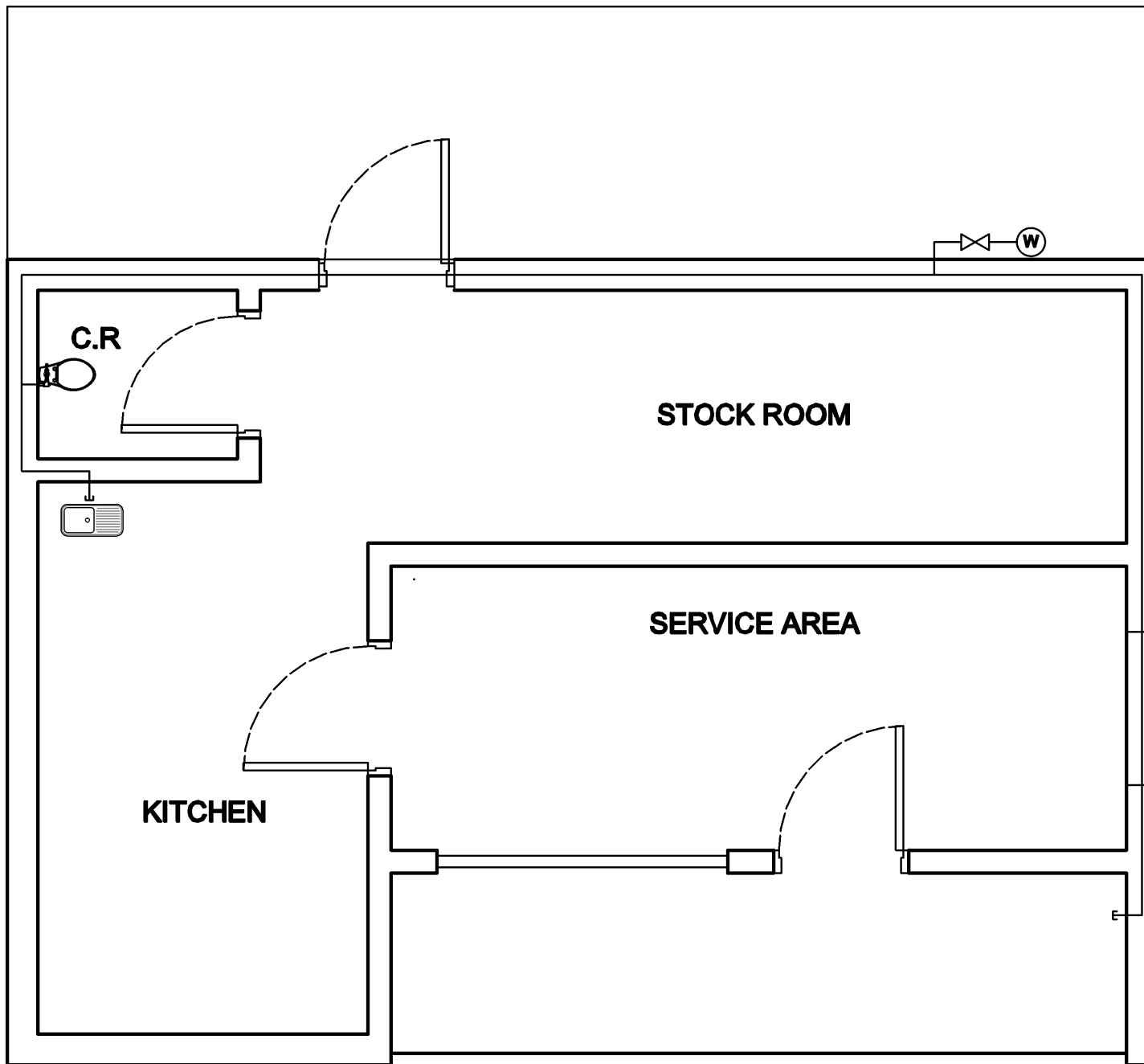
WATER-LINE LAY OUT
